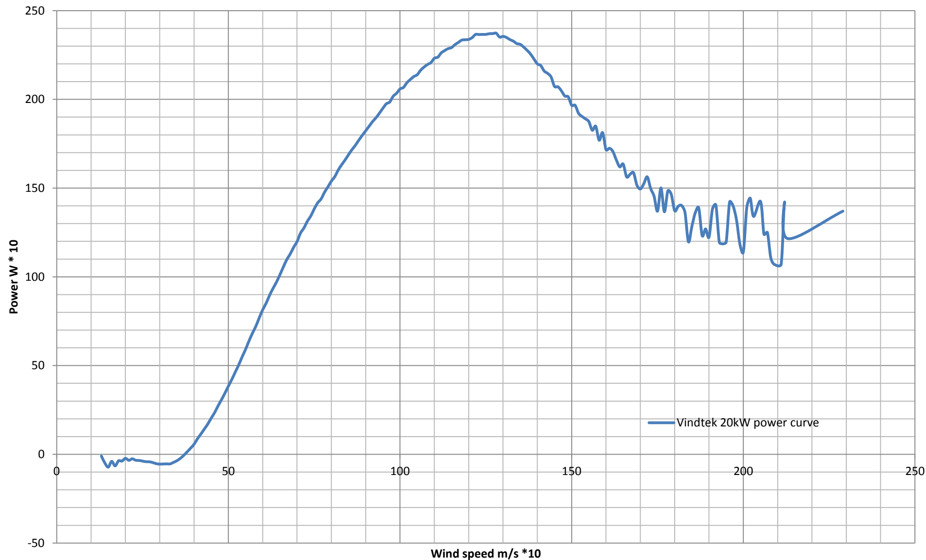
Vindtek 20kW power curve
